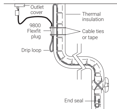
Figure 1. Typical manufactured housing installation
