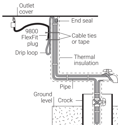
Figure 6. Multiple run installation
